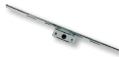
Espagnolette 20mm Backset 8mm 2 cam 800mm Part Number: S5184 Box Quantity: 50
