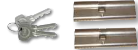
E63: Anti-Bump Keyed Alike Cylinders 40/50 Nickel Part Number: S9813AB Box Quantity: 5 Pairs
