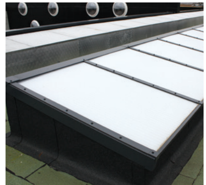
Em-Glaze continuous polycarbonate rooflight
