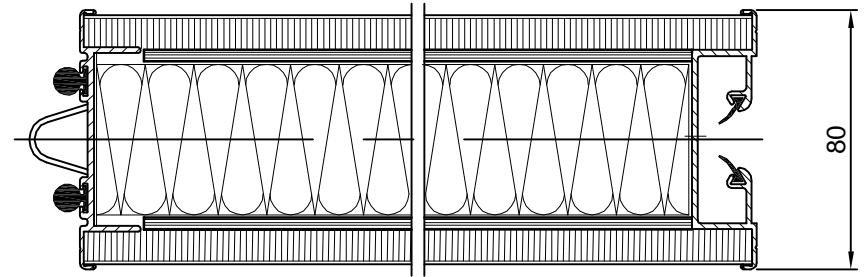
a) Exposed edge profile
