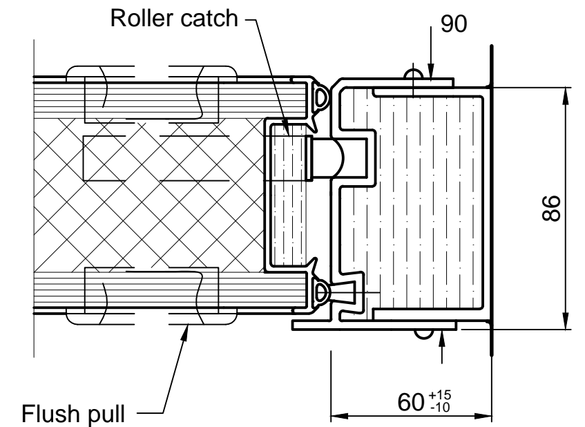
HORIZONTAL SECTION - WALL JAMBS
