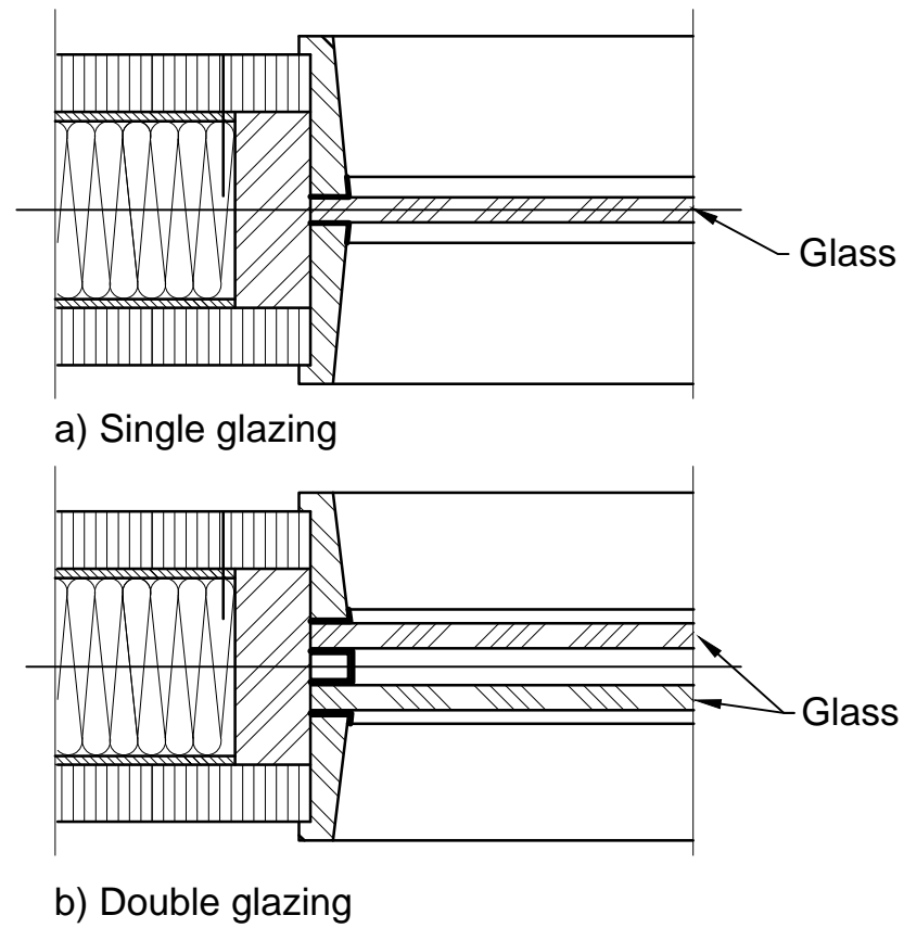
5. HORIZONTAL GLAZING SECTIONS
