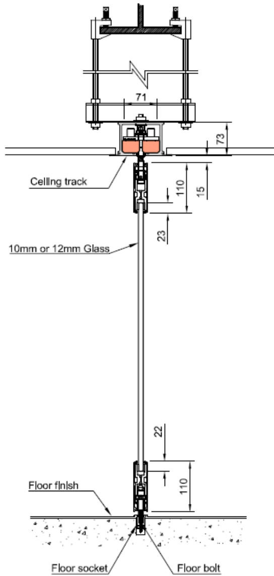
VERTICAL SECTION OF PANEL & TRACK FIXING
