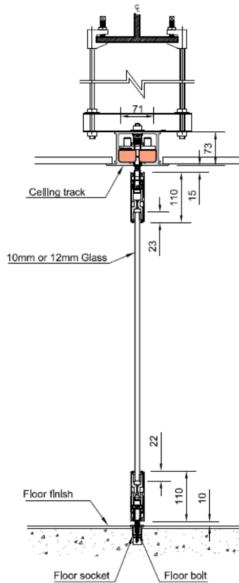
VERTICAL SECTION OF PANEL & TRACK FIXING
