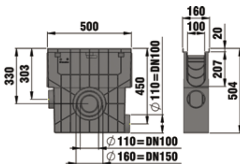
Trash box with PE mud bucket and Slotted grating SW 80/10, cl. A 15, locked
