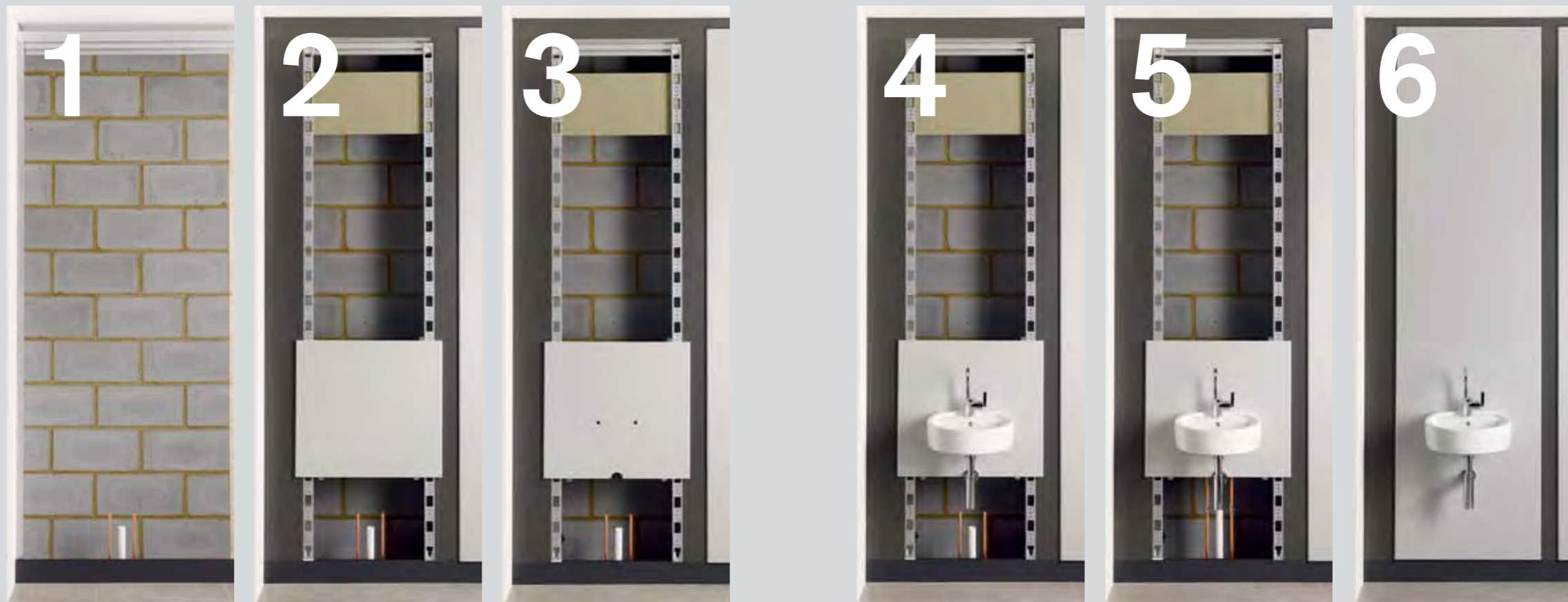
01 Once the site has been prepared, fix the aluminium site frame to the wall, ceiling and floor.
