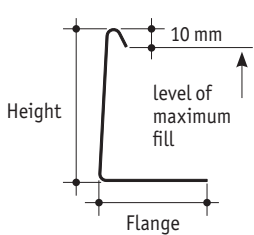
gravel-protection strip 70
