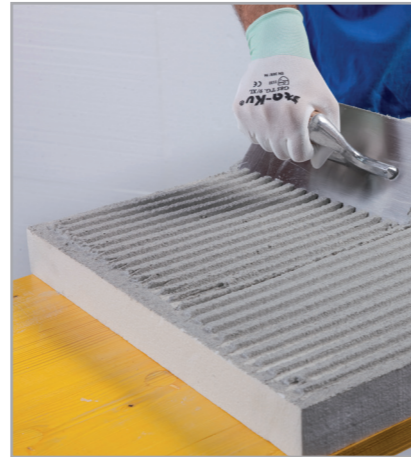
Spread an even layer of adhesive on the back of the insulating panel
