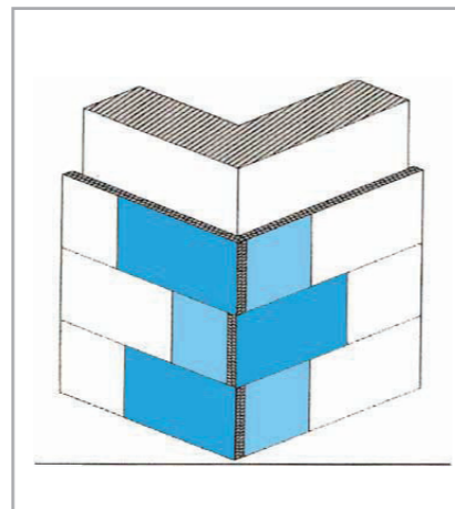
Typical corner section insulation boards
